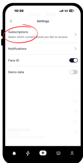
Step 2 Subscriptions
